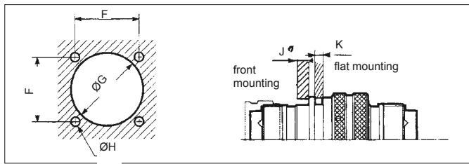
panel cut-out
